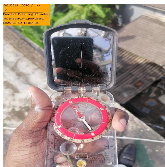
Mobitel Existing RF antenna azimuth sector 01
