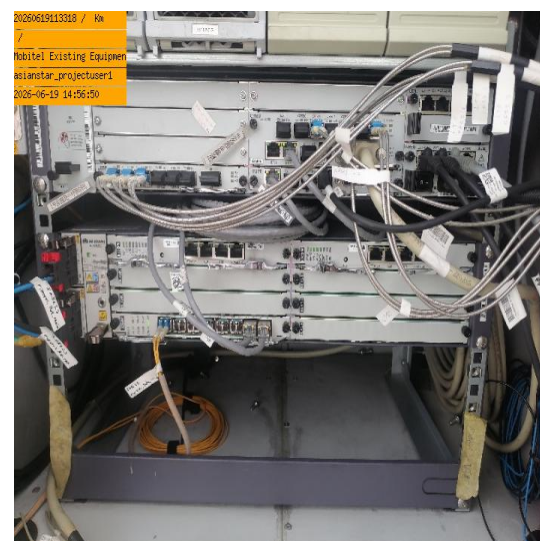
Mobitel Existing Equipment detail In look 4
