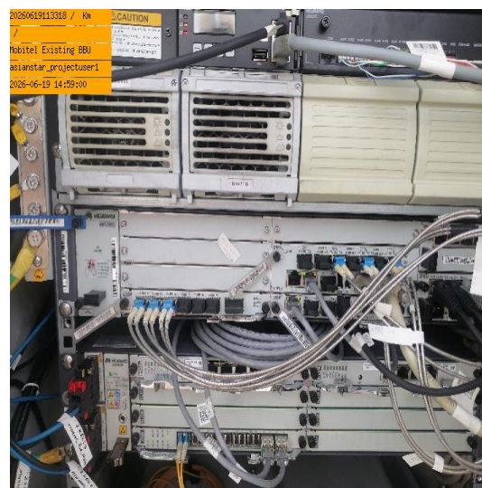
Mobitel Existing BBU
