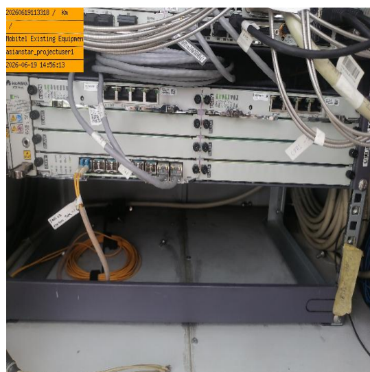
Mobitel Existing Equipment detail In look 3
